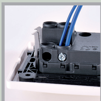
DIFFERENT WIRES ON THE SAME TERMINAL
